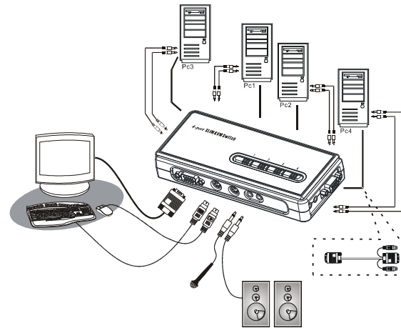
Configuration Diagram
